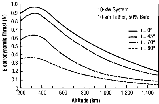
Fig. 4 Estimated propulsive performance of an upper-stage demonstrator vehicle using EDT thrust.
