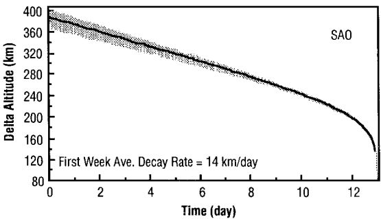
Fig. 1 Electrodynamic tether dramatically reduces the orbital lifetime of the upper stage.
